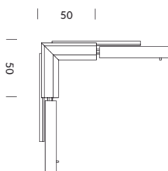
4 L joint wall-ceiling + electrical connector
