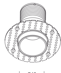
zermatt 7 CUT OUT Ø60 mm MIN. HEIGHT 95 mm
